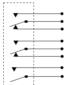
N/O Com N/C ALARM 1 (Fitted as standard) N/O Com N/C ALARM 2 N/O Com ALARM 3
