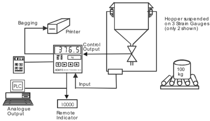
Figure 1.2 Drum Filling
