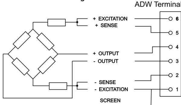
ADW Terminal Block
