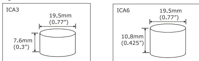
Figure 2.1 Dimensions
