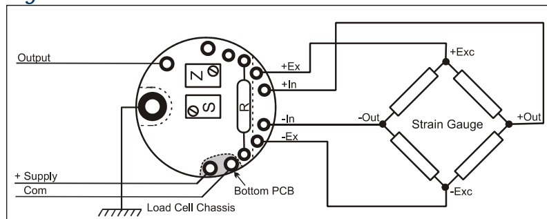
Figure 2.3 Connection Details for the ICA6
