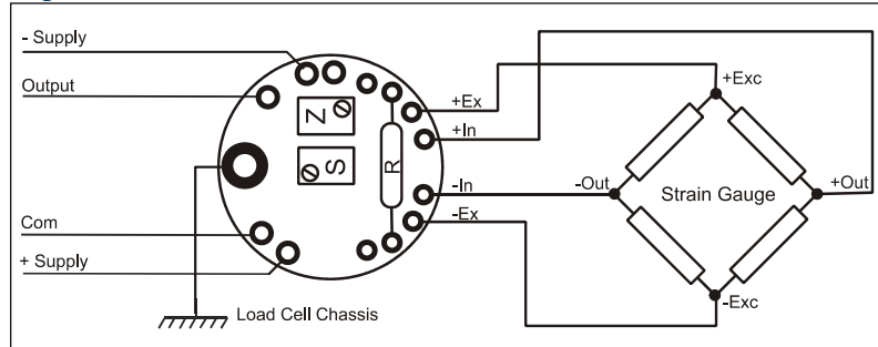
Figure 2.2 Connection Details for the ICA3
