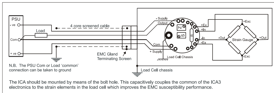
Figure 2.4 Connection Details for Best EMC Immunity
